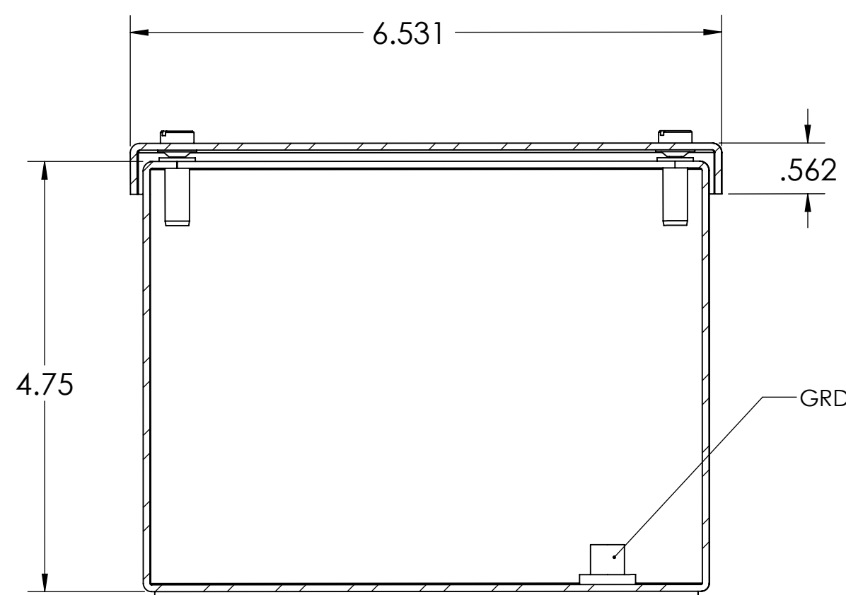
SECTION F-F SCALE 1 : 1.5
