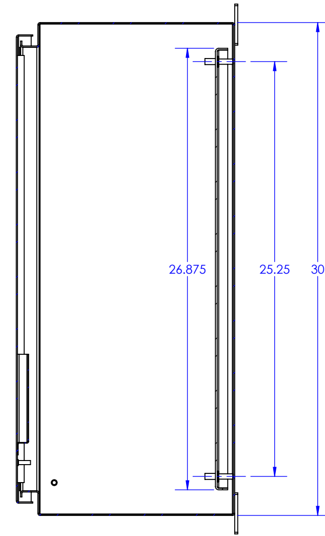
SECTION C-C
