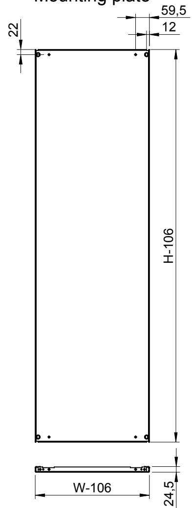
Mounting plate
