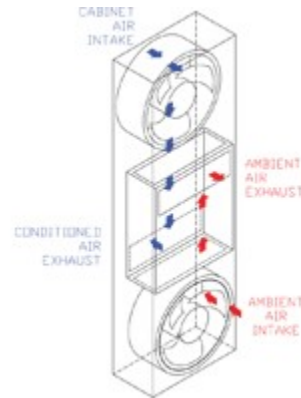
Counter Flow
