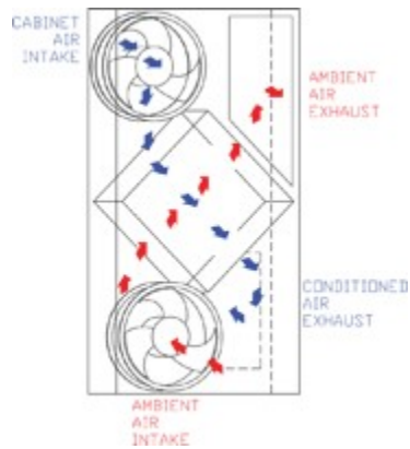
Cross Flow
